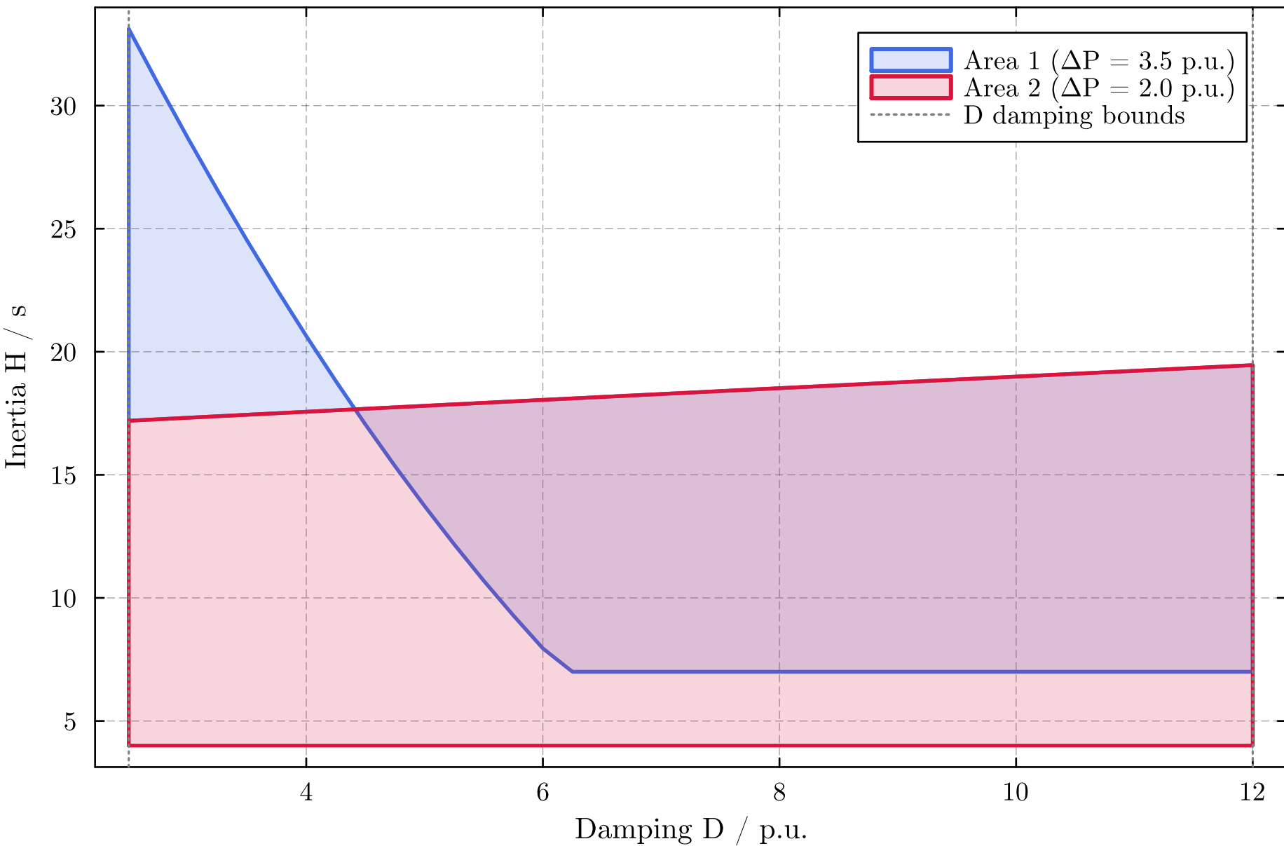
Multi-Area Feasible Region Comparison (Overlay)
